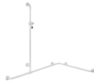
Rail with vertical support bar and shower head holder 1100 x 762 x 762 mm / 1100 x 962 x 962 mm 801.35.3 ...
