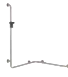
Shower grab rail with vertical support bar and shower head holder W 762 x H 1100 x D 762 mm 805.35.210 ...
