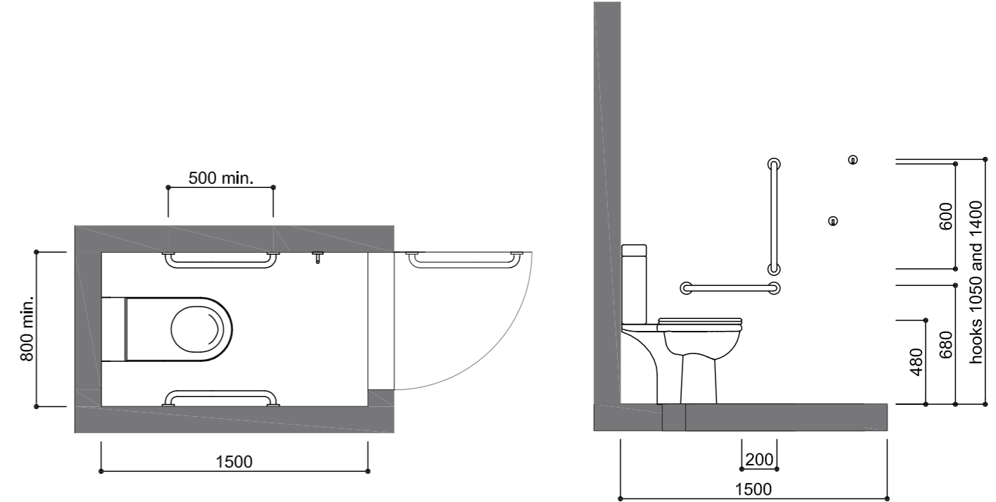
WC cubicle for ambulant disabled people
