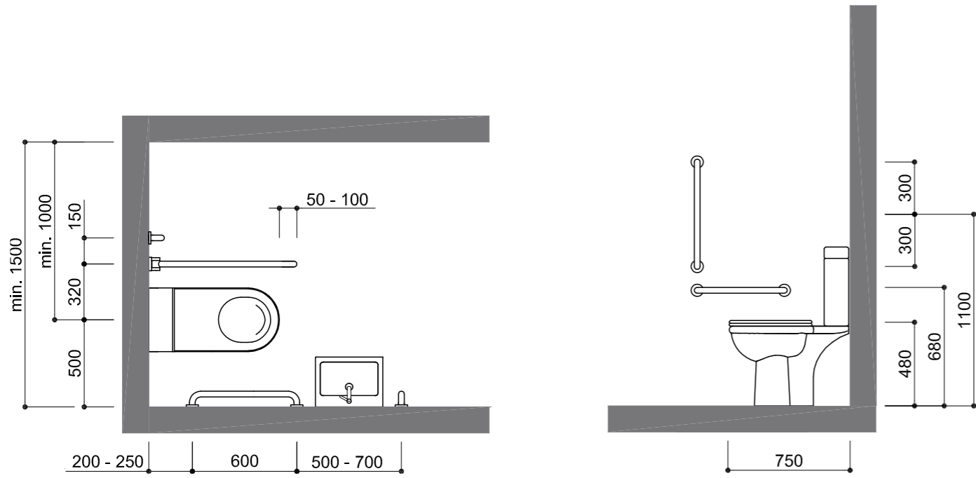
WC cubicle for wheelchair access
