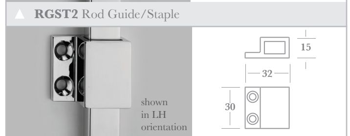
▲ RG2 Rod Guide (reversible for LH or RH use)
