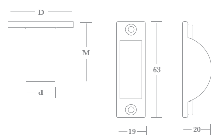
▲ 0604 Easy Clean Socket supplied with finish matched screws & rawl plugs
