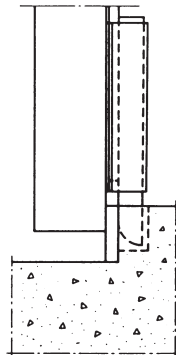
Flat iron connection Bolt 2548 Receiver not necessary
