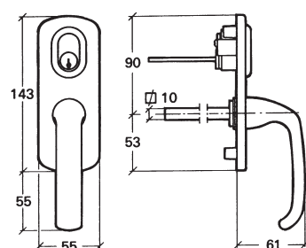
Outer handle 664
