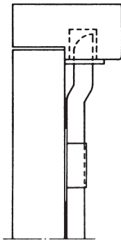
Outward-opening, wooden frame Receiver 351
