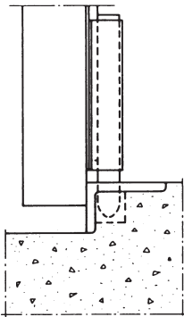
Angled iron connection Bolt 2547 Receiver not necessary
