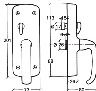
Inner lock housing 280
