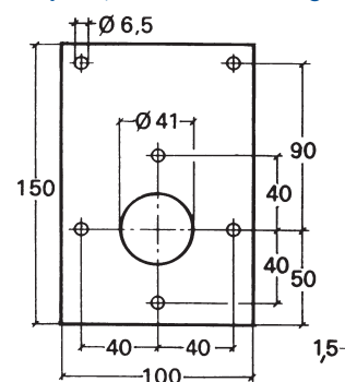
Cover plate, inner lock housing 1126
